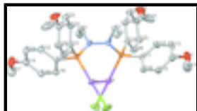
Fig. 1. Molecular structure of the title complex drawn with displacement ellipsoids at the 50% probability level. Hydrogen atoms and solvent THF have been omitted for clarity.
